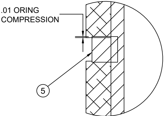
DETAIL D
