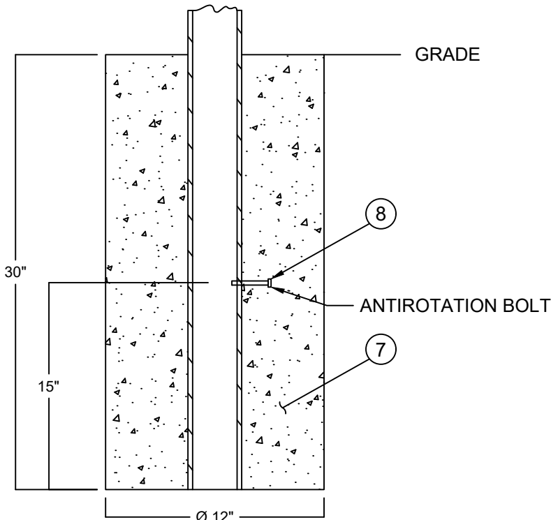
DETAIL E
